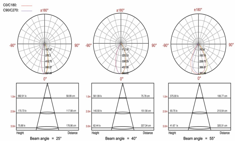
Light intensity distribution curve
